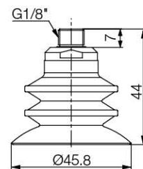
[ With 18M fitting ]
